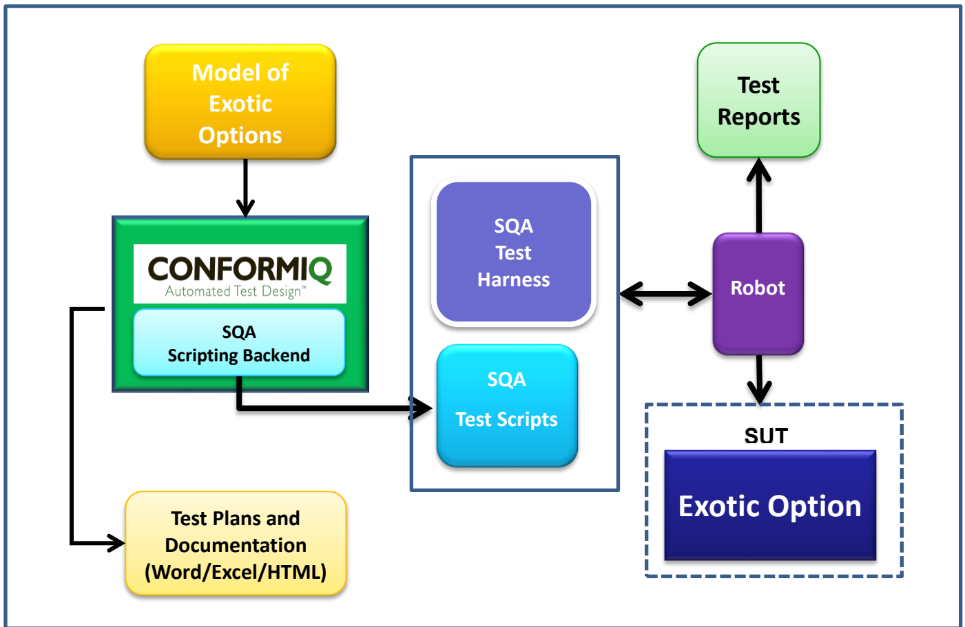
Figure 3 – Test System Architecture
